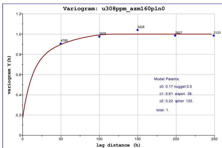
Figure 108: Along-strike variogram, Detail 2 domain 1
