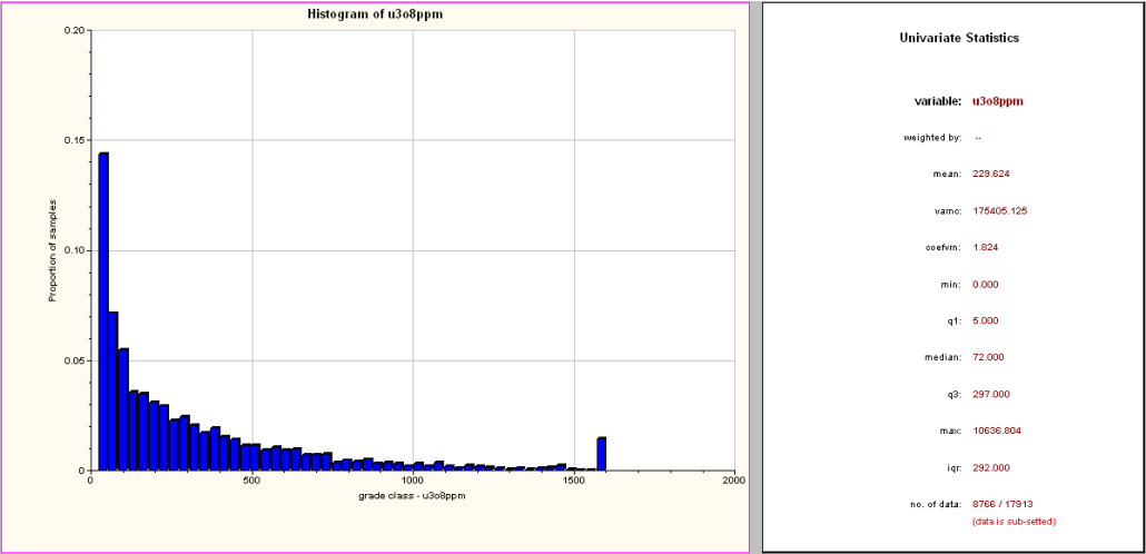
Figure 76: Histogram of grades in Detail 1, domain 1, above the water table, including clustered data
