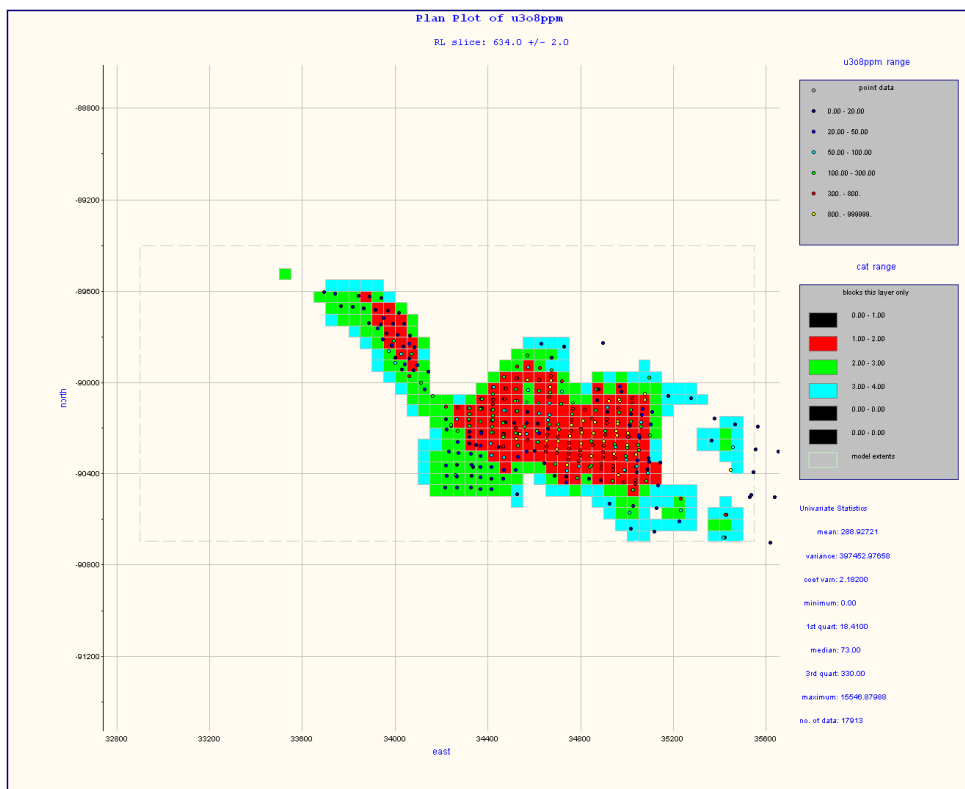
Figure 159: Detail 1 632-636RL, panel confidence categories
