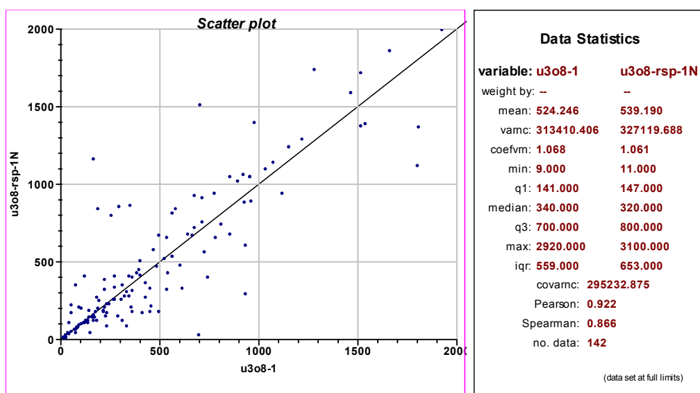
Figure 39: U_3O_8 grades in re-splits of Gencor percussion drill samples
