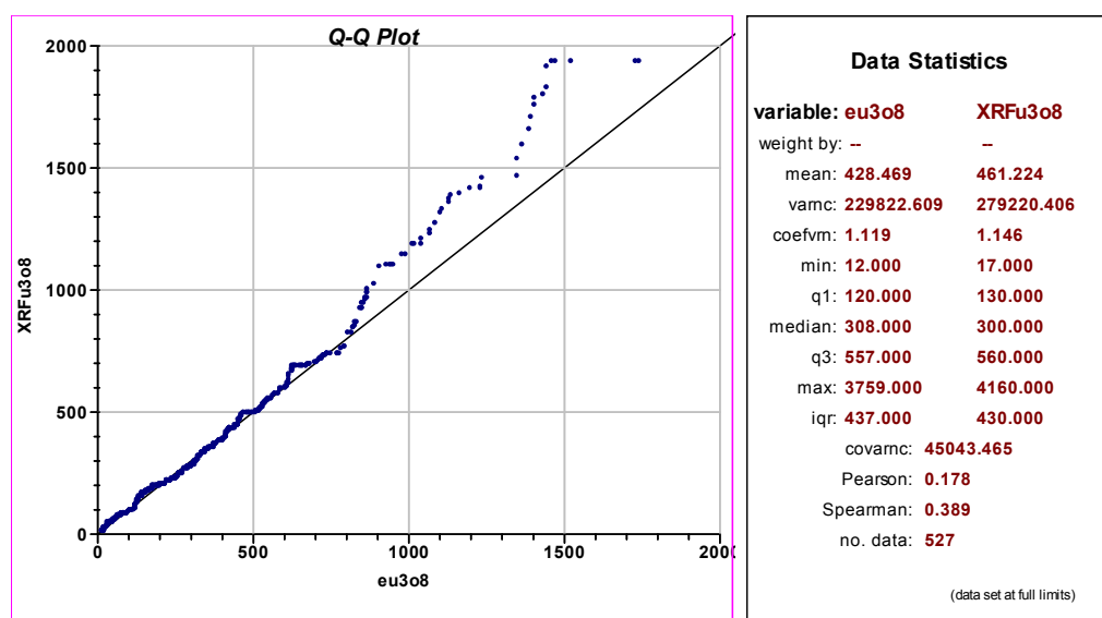
Figure 51: Gencor XRF assays versus nearest-neighbour Acclaim radiometric grades
