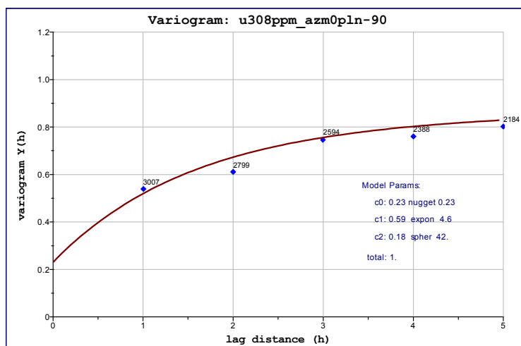
Figure 113: Down-hole variogram, Detail 3
