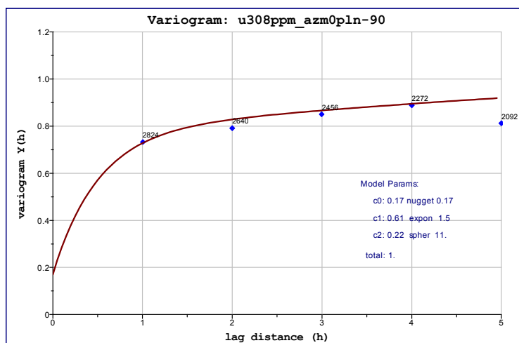
Figure 107: Down-hole variogram, Detail 2 domain 1
