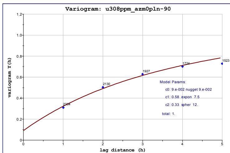
Figure 122: Down-hole variogram, Detail 5 domain 2
