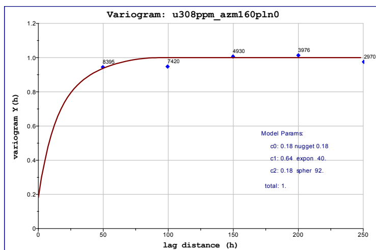
Figure 111: Along-strike variogram, Detail 2 domain 2
