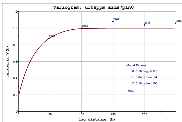
Figure 112: Across-strike variogram, Detail 2 domain 2
