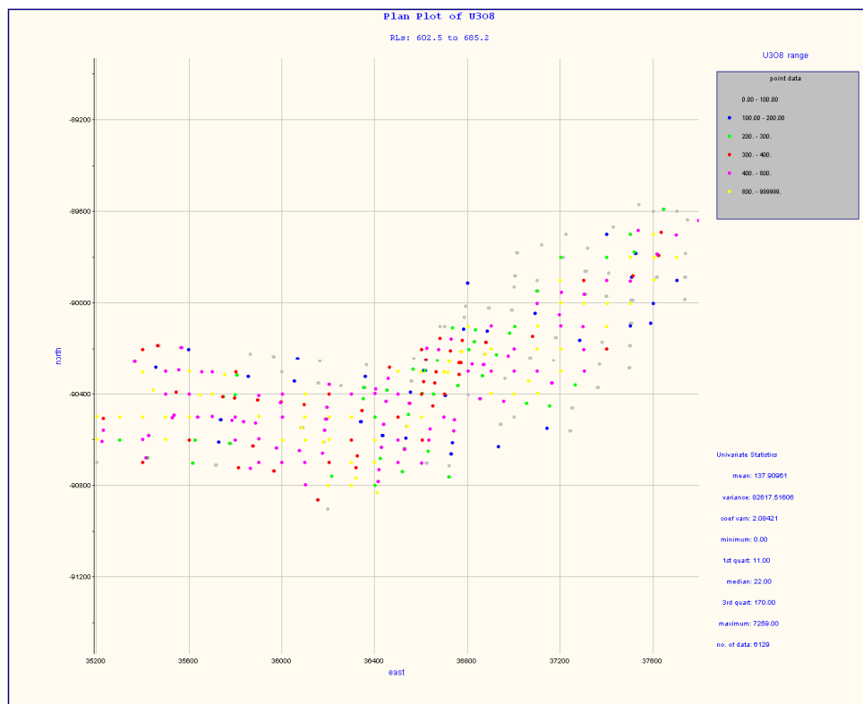
Figure 70: Sample composites in Detail 5
