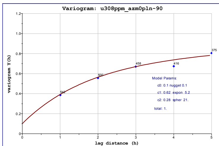
Figure 125: Down-hole variogram, Detail 6
