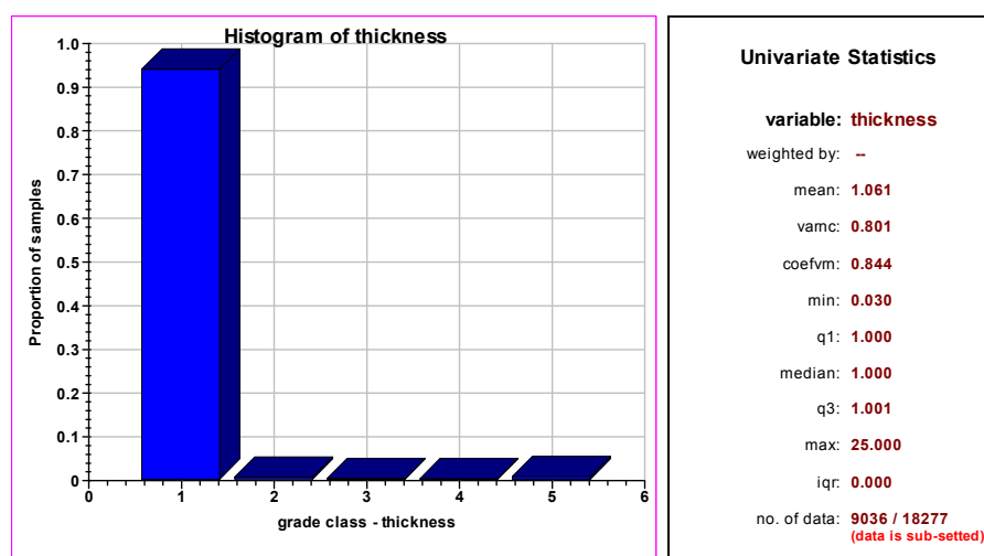
Figure 59: Lengths of Gencor native sample intervals with U_3O_8 assays, Detail 1
