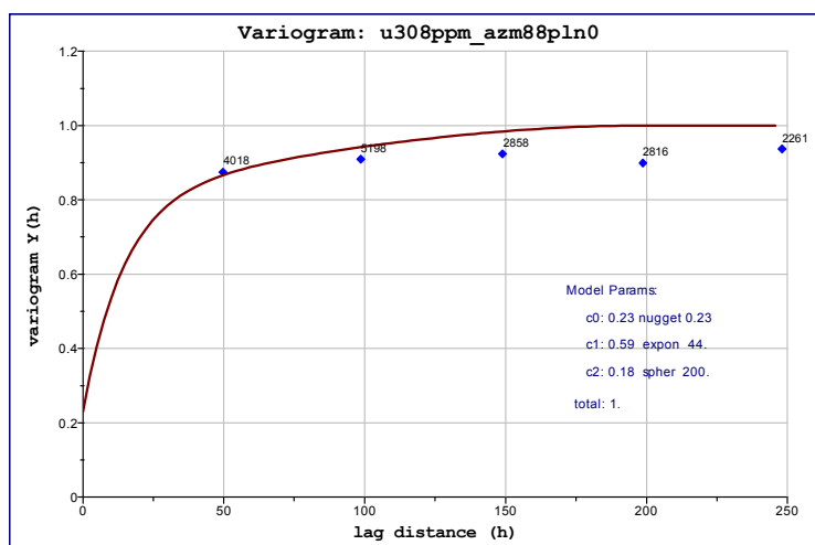
Figure 115: Across-strike variogram, Detail 3
