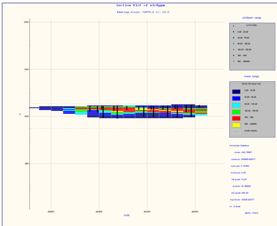
Figure 166: Detail 1 section 34975E, mean U_3O_8 grades
