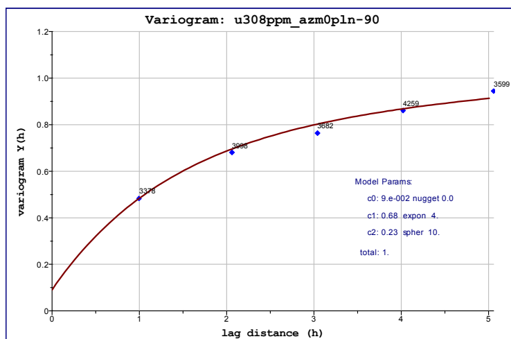
Figure 104: Down-hole variogram, Detail 1 domain 1
