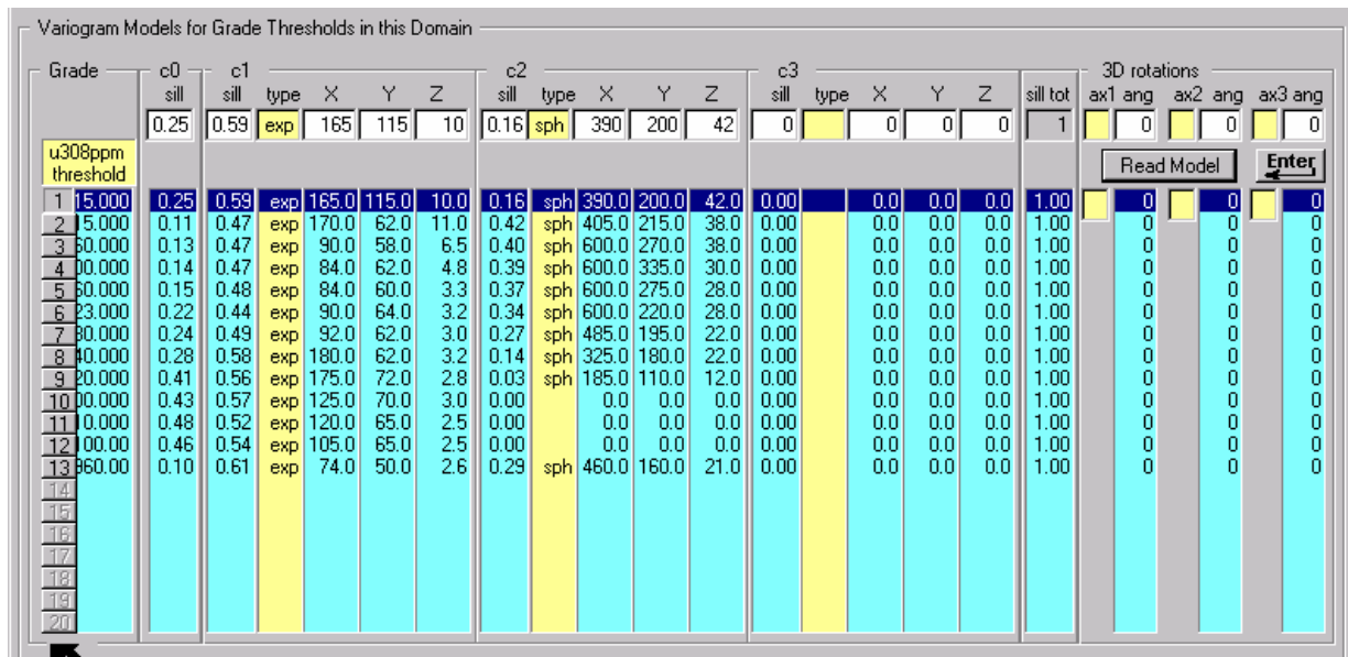
Figure 139: U_3O_8 and indicator variogram models applied to Detail 4
