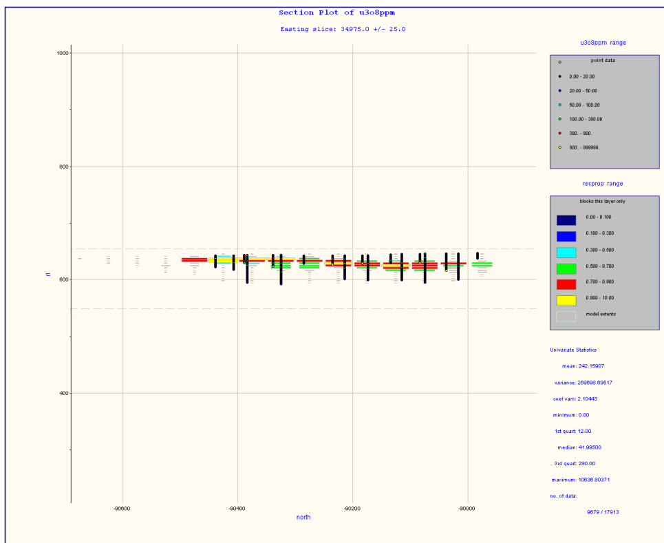
Figure 167: Detail 1 section 34975E, recoverable proportions at 0.25kg/t U_3O_8 cut-off
