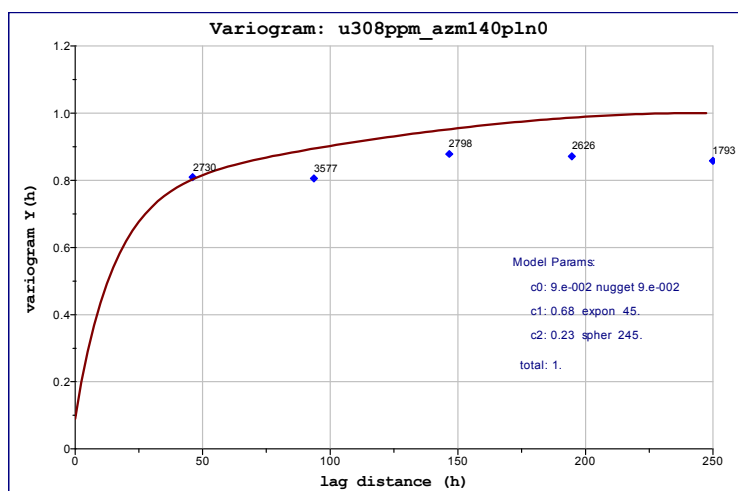
Figure 105: Along-strike variogram, Detail 1 domain 1
