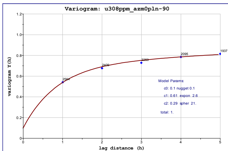
Figure 116: Down-hole variogram, Detail 4
