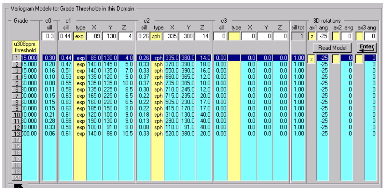
Figure 140: U_3O_8 and indicator variogram models applied to Detail 5, domain 1
