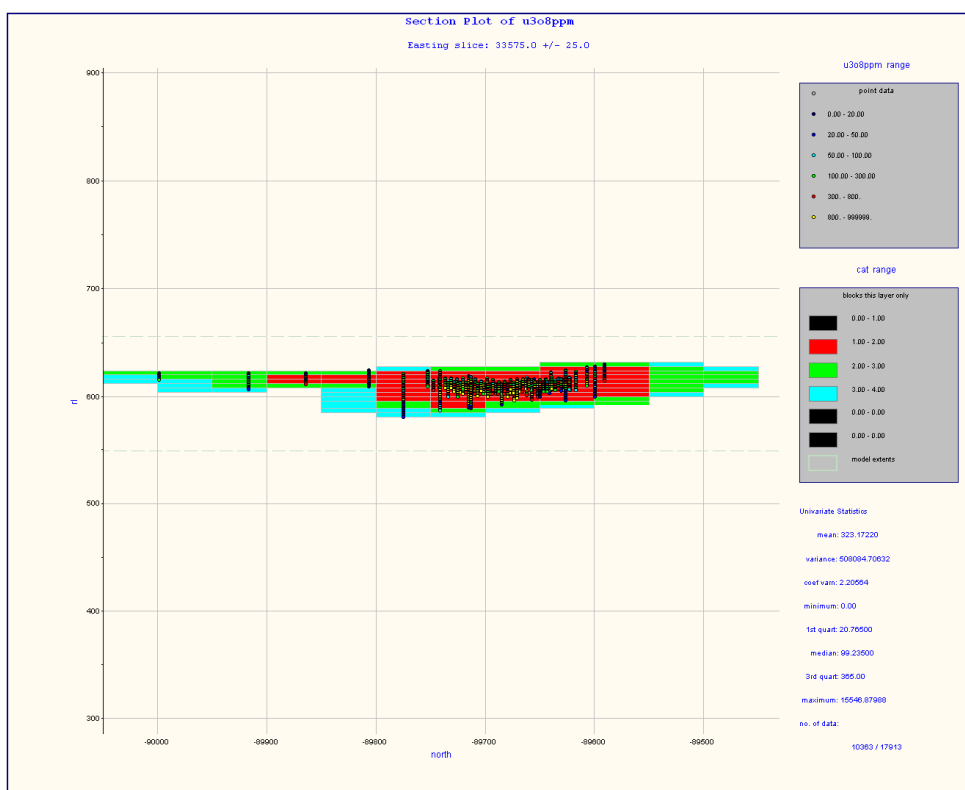
Figure 168: Detail 1 section 33575E, panel confidence categories
