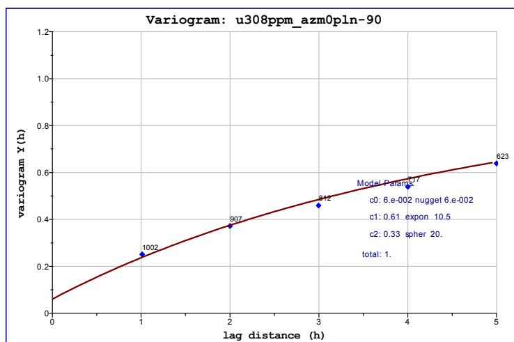
Figure 119: Down-hole variogram, Detail 5 domain 1
