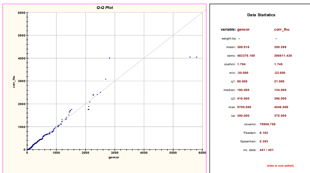
Figure 56: U_3O_8 grades in wet Gencor percussion drill samples and nearby Paladin gamma logs
