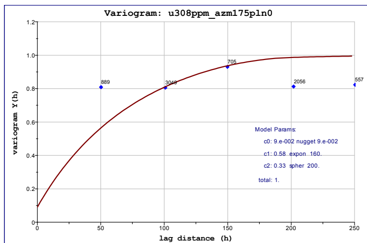
Figure 123: Along-strike variogram, Detail 5 domain 2
