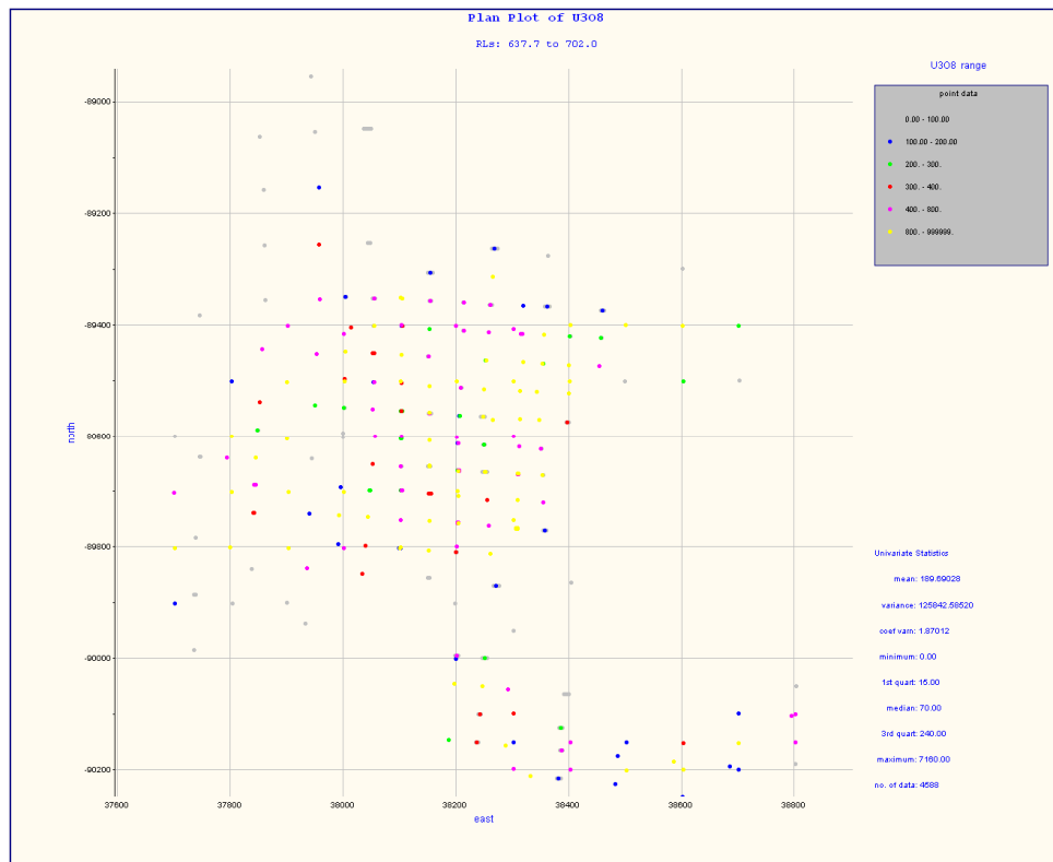
Figure 68: Sample composites in Detail 3
