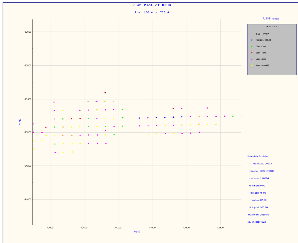
Figure 69: Sample composites in Detail 4
