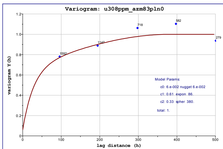
Figure 121: Across-strike variogram, Detail 5 domain 1
