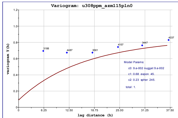
Figure 132: Variogram using mine drilling only, along-strike direction
