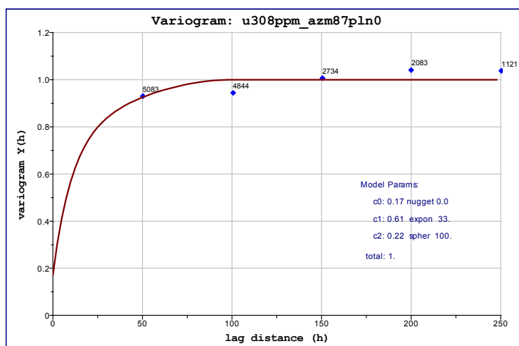
Figure 109: Across-strike variogram, Detail 2 domain 1
