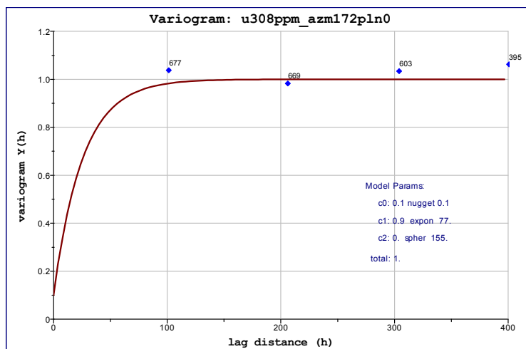
Figure 129: Along-strike variogram, Detail 7
