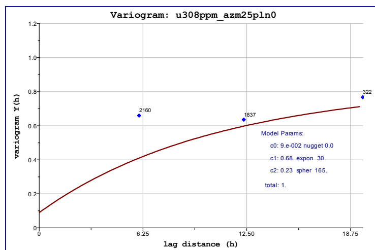
Figure 133: Variogram using mine drilling only, across-strike direction
