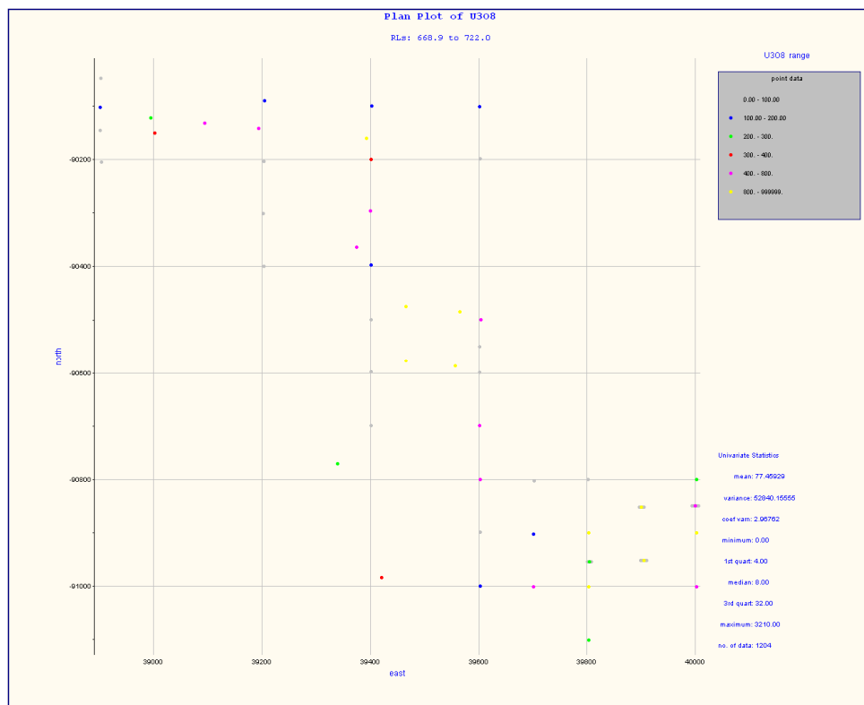
Figure 71: Sample composites in Detail 6
