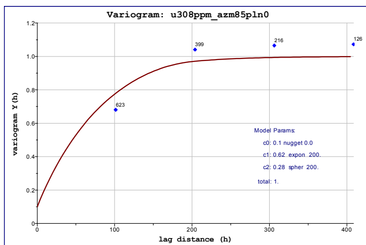
Figure 127: Across-strike variogram, Detail 6
