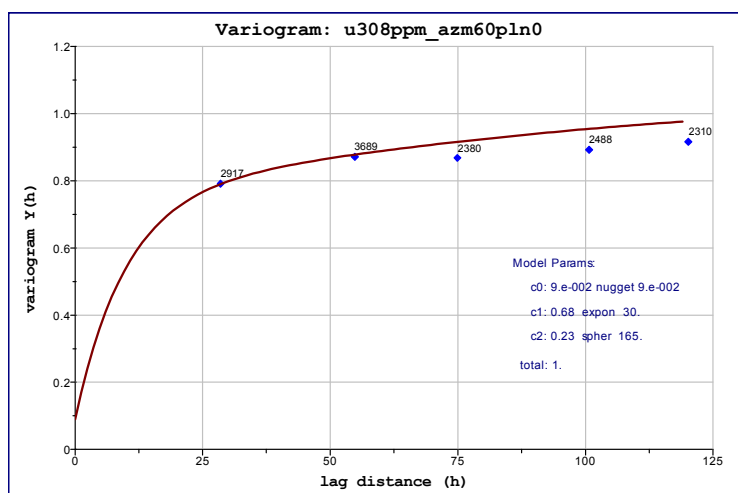
Figure 106: Across-strike variogram, Detail 1 domain 1
