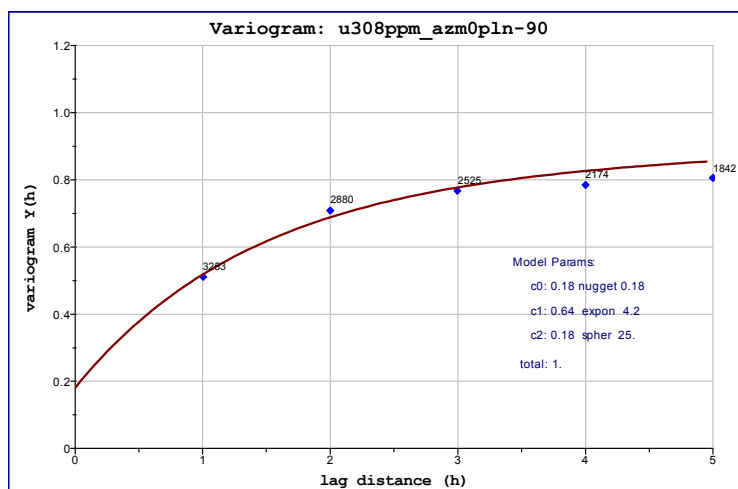
Figure 110: Down-hole variogram, Detail 2 domain 2
