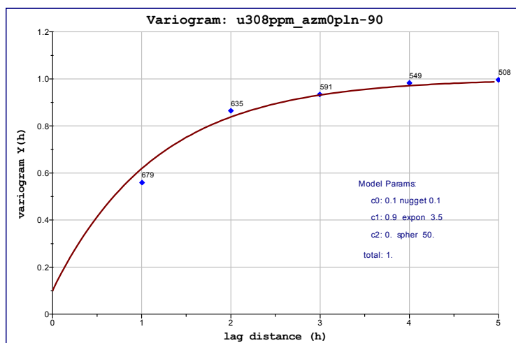
Figure 128: Down-hole variogram, Detail 7
