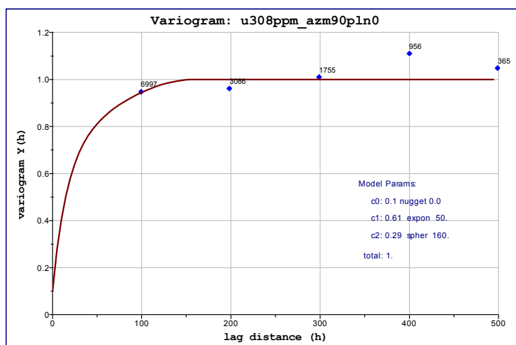
Figure 118: Across-strike variogram, Detail 4
