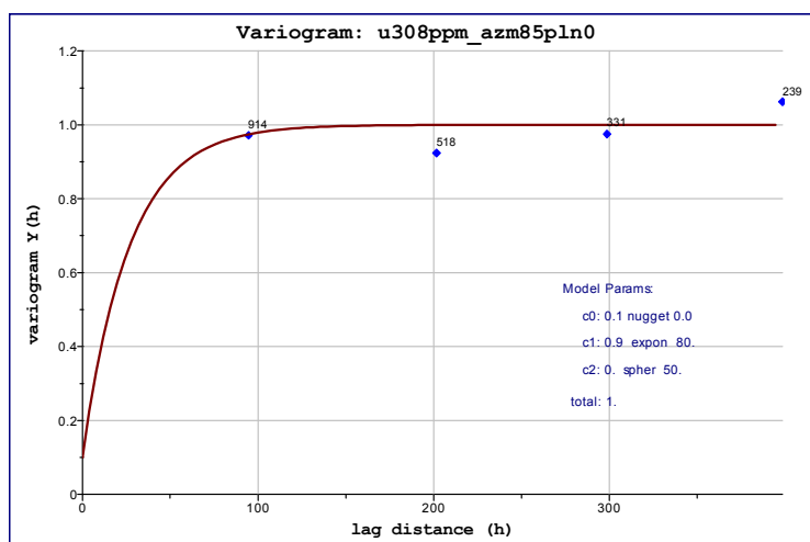
Figure 130: Across-strike variogram, Detail 7
