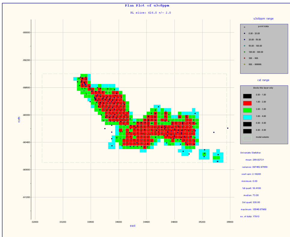
Figure 158: Detail 1 624-628RL, panel confidence categories
