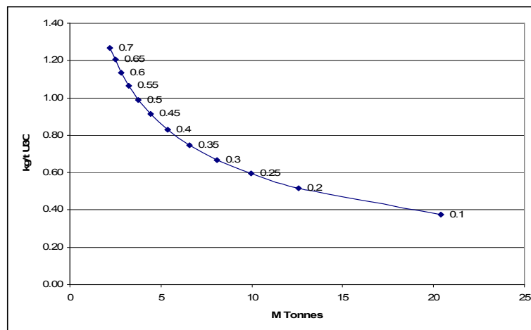
Figure 145: Grade-tonnage curve for measured and indicated resources, Detail 2
