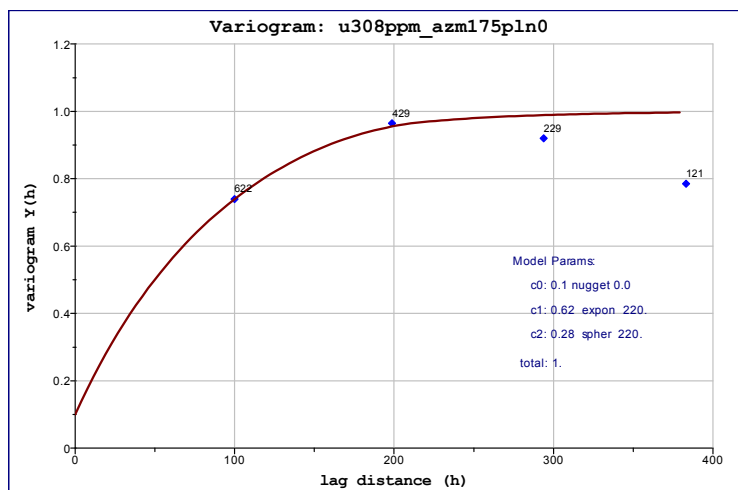
Figure 126: Along-strike variogram, Detail 6
