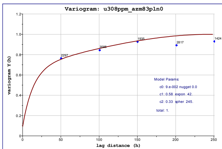
Figure 124: Across-strike variogram, Detail 5 domain 2
