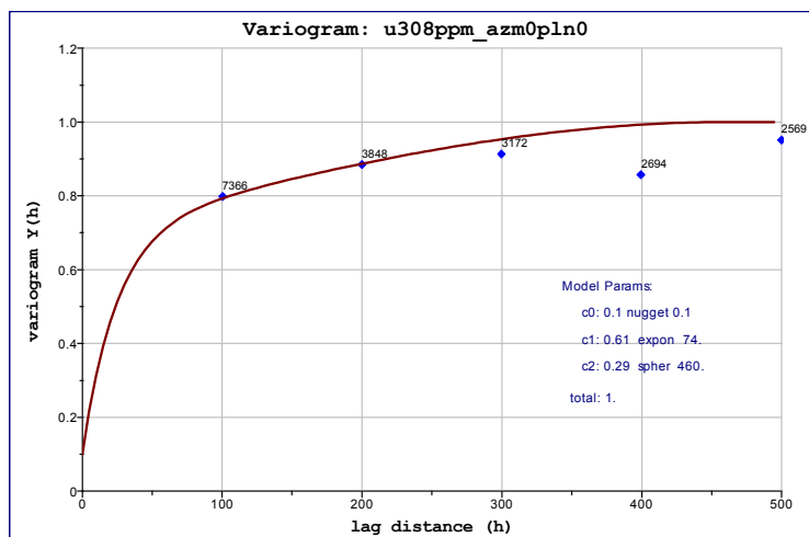
Figure 117: Along-strike variogram, Detail 4
