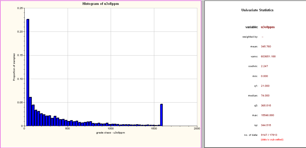
Figure 77: Histogram of grades in Detail 1, domain 1, below the water table, including clustered data
