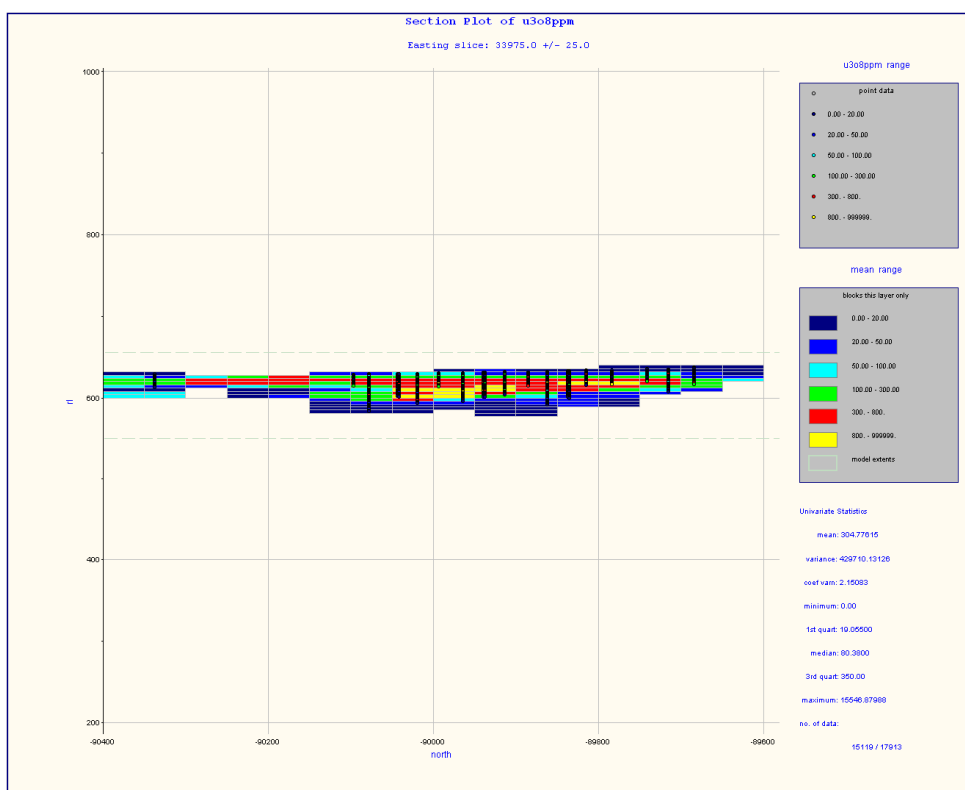
Figure 162: Detail 1 section 33975E, mean U_3O_8 grades
