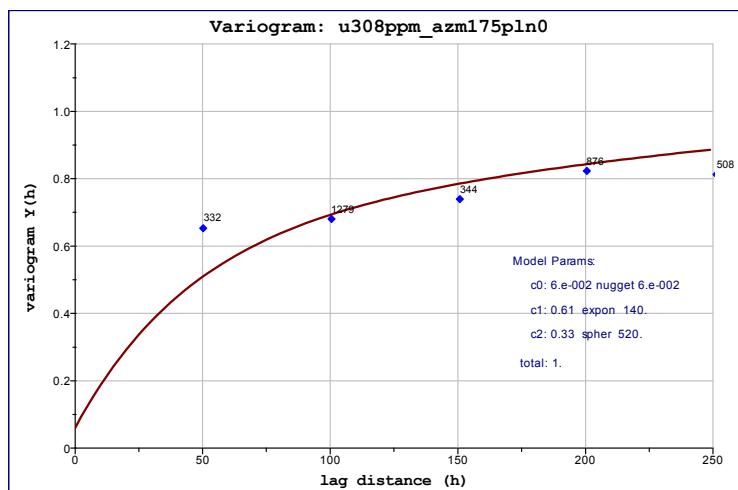
Figure 120: Along-strike variogram, Detail 5 domain 1
