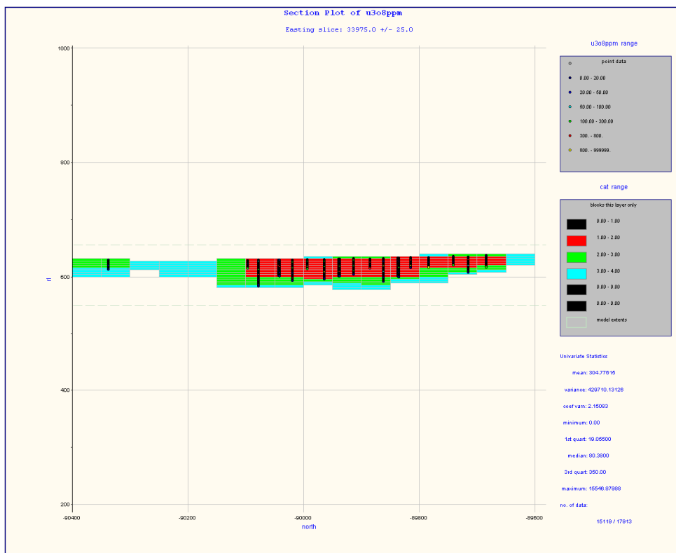
Figure 169: Detail 1 section 33975E, panel confidence categories
