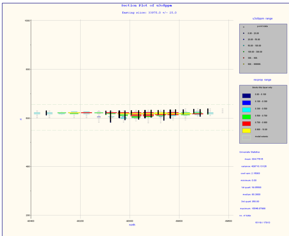
Figure 163: Detail 1 section 33975E, recoverable proportions at 0.25kg/t U_3O_8 cut-off
