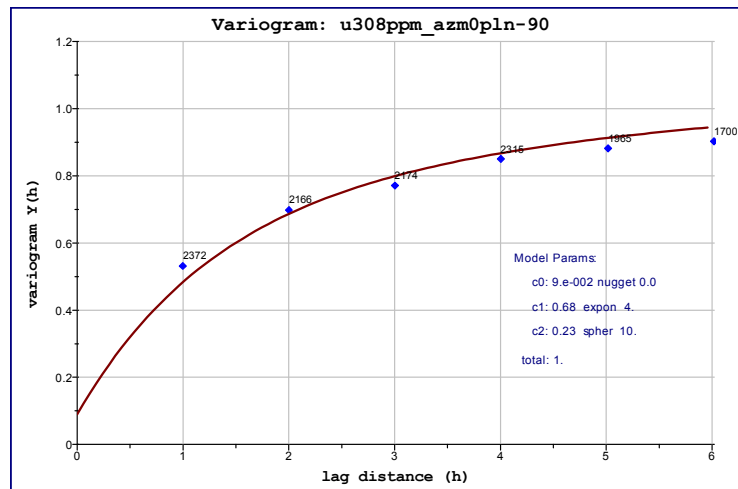
Figure 131: Variogram using mine drilling only, vertical direction
