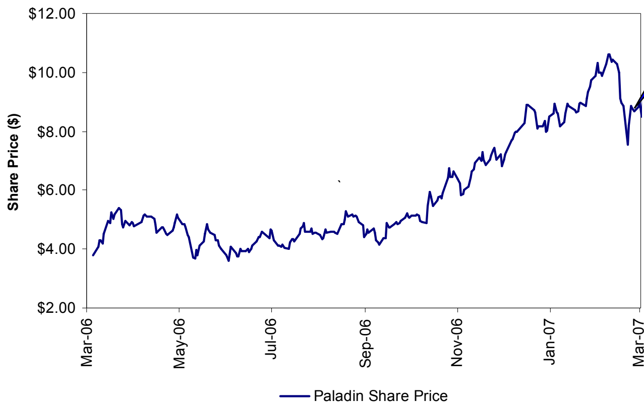
Paladin Daily Closing Share Price (ASX)
