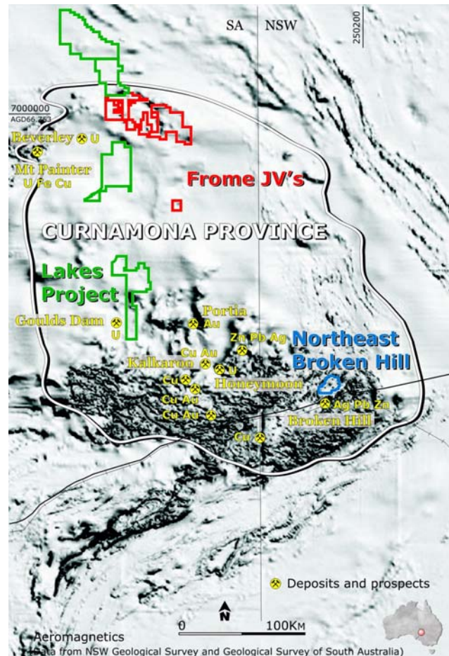
[Figure 4] Curnamona Province: greyscale magnetic image showing Red Metal projects locations and the major deposits and prospects of the region
